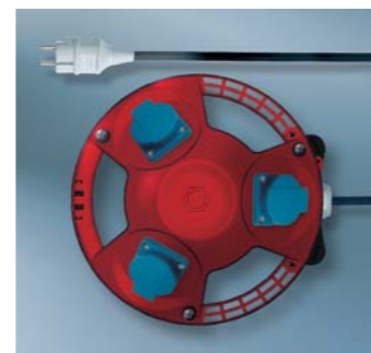
3 SCHUKO® sockets 16A, 230V with 3 m of supply cable H07RN- F5G1.5 with SCHUKO® plug 16A, 230V Ref. no. 94357
