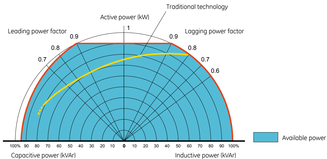
SG-CE Series 160 - 300 kVA power capability
